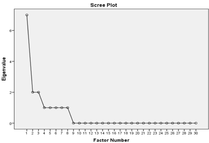
Figure 2. The scary graph of factors' number determination
