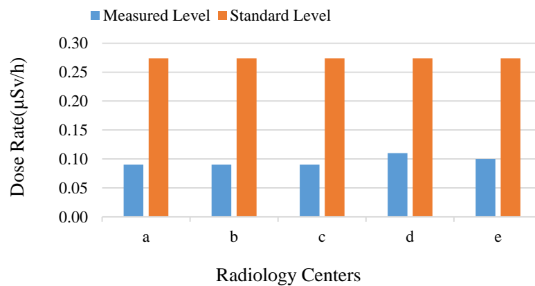
Figure 2. Comparison of measured radiation dose outdoor radiological centers and world standard level
