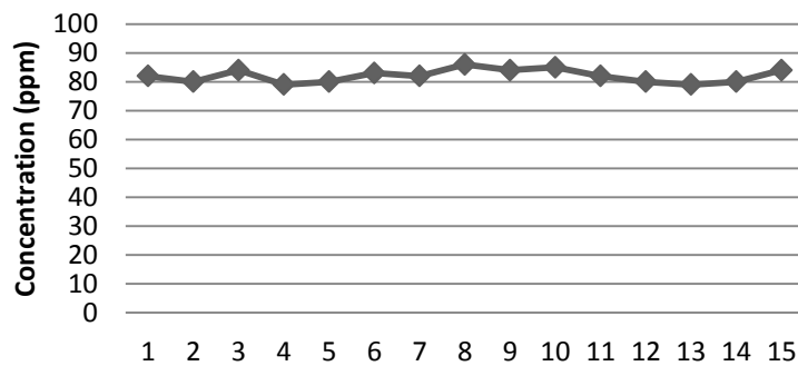
Figure 4. Benzene concentrations measured during 15 repeated tests in same conditions
