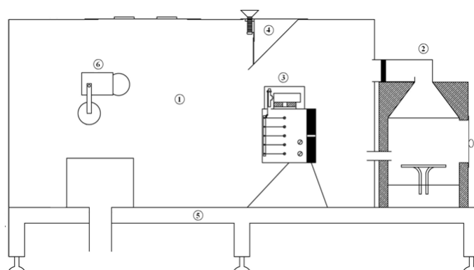
Figure 2: Schematic diagram of airborne pollutant simulation chamber (1. Main chamber, 2. Warming chamber, 3. Blowing system, 4. Evacuation funnel, 5. Platform, 6. Filament lamp)
